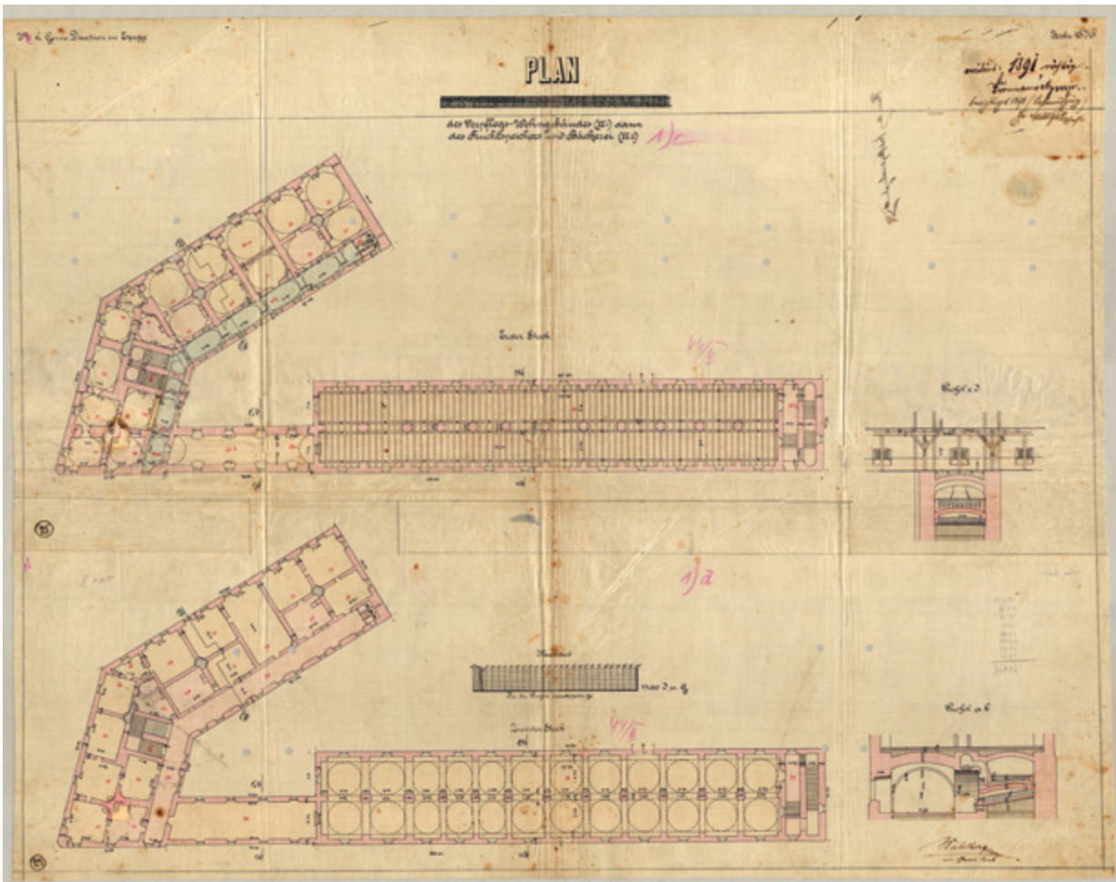
SI. 8. Plan Opskrbne vojarne, žitnice i pekare, prvi i drugi kat, 1876. (Državni arhiv u Osijeku) Layout of the Supply Barracks, granary and bakery, 1 st and 2 nd floors, 1876 (State Archives in Osijek)
